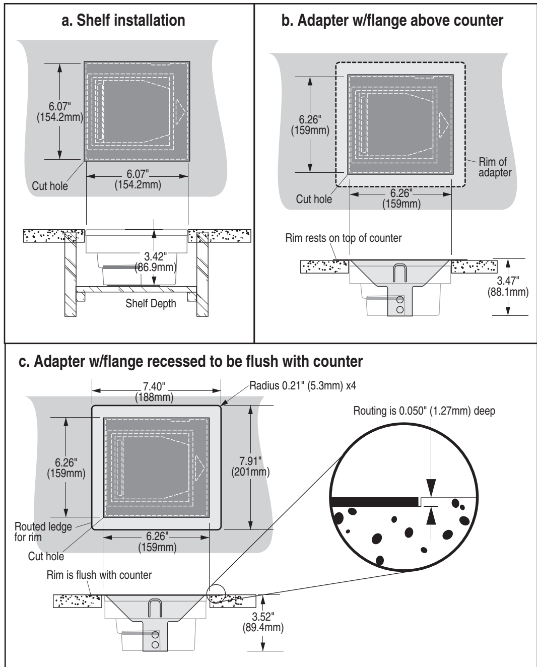
Figure 3. Countertop Cutouts
